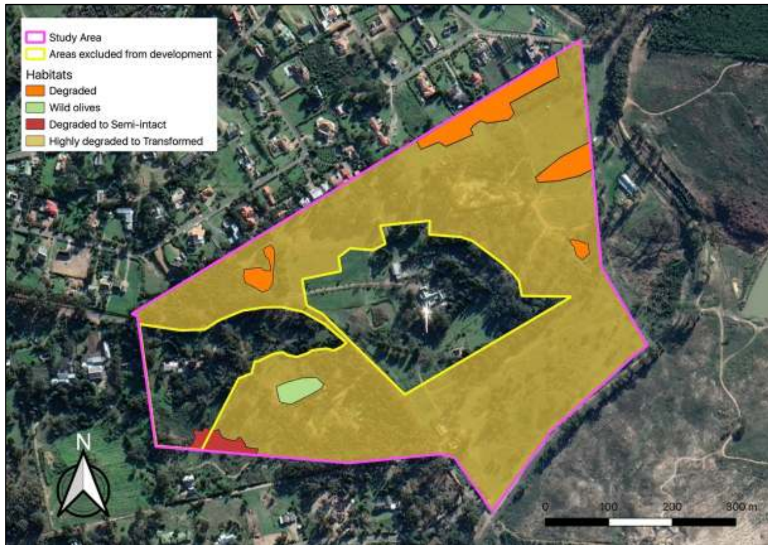
Figure 9. HABITAT MAP: Google Earth™ aerial image showing the habitats mapped within the Study area.
