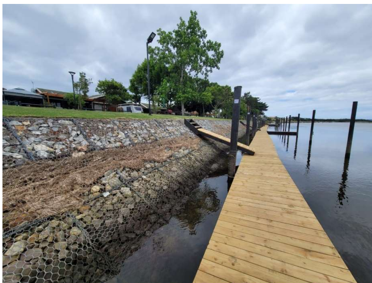
Jetty installation progress (photographs taken 28 November 2023)
