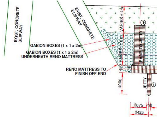
Upstream extension of the toe of the Reno-matress as described above (MOSOMO, 2019)
