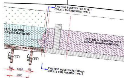
Upstream extension of the toe of the Reno-matress as described above (MOSOMO, 2019)
