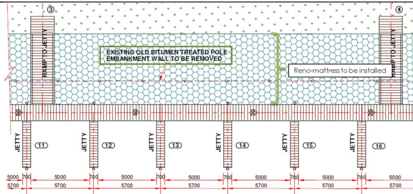
Reno-matress that was installed and the line of the existing embankment wall (MOSOMO, 2019)
