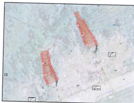
Figure 10: Plan view of stepped gabion hydraulic structures terminating at a non-perennial stream of the Meul River (Site 69).
