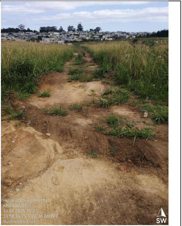
Eroded areas have been covered with topsoil and rows of sandbags/small soil berms have been installed.
